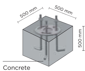
AC053 - Base Plate
